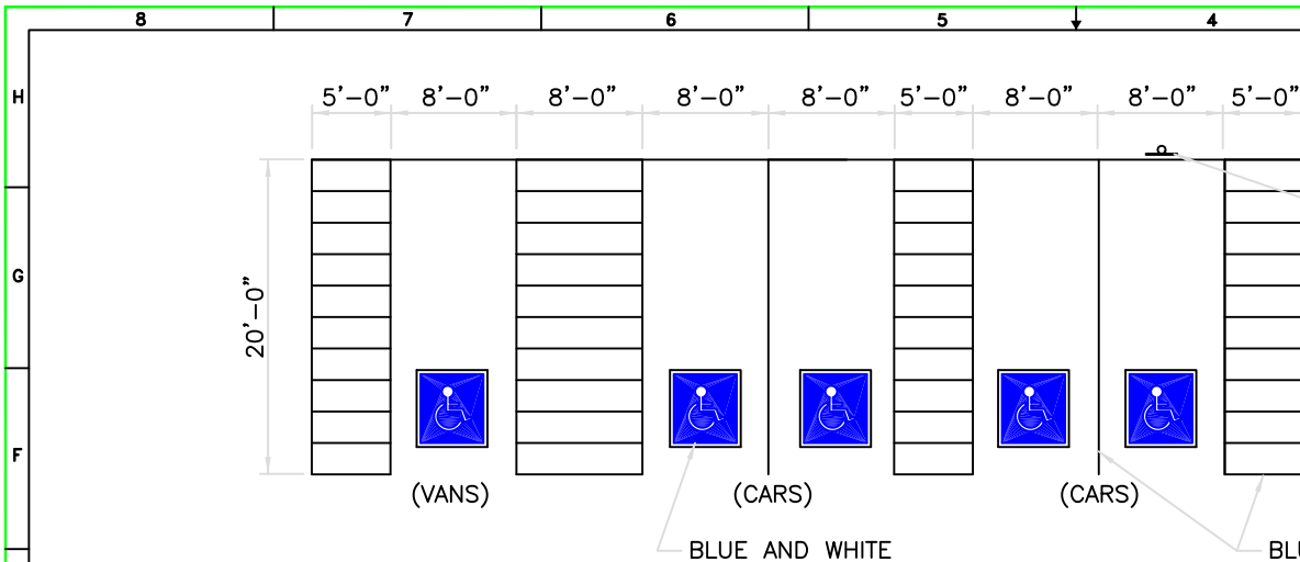
ACCESSIBLE PARKING LAYOUT SCALE: NONE
