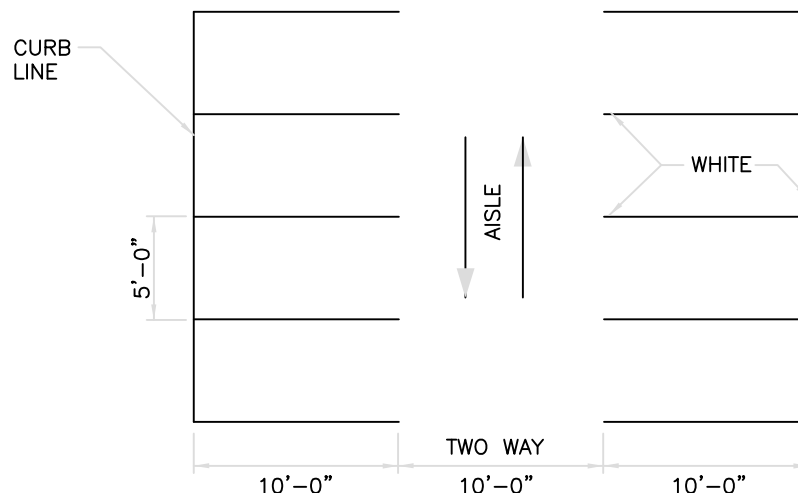
MOTORCYCLE PARKING LAYOUT SCALE: NONE
