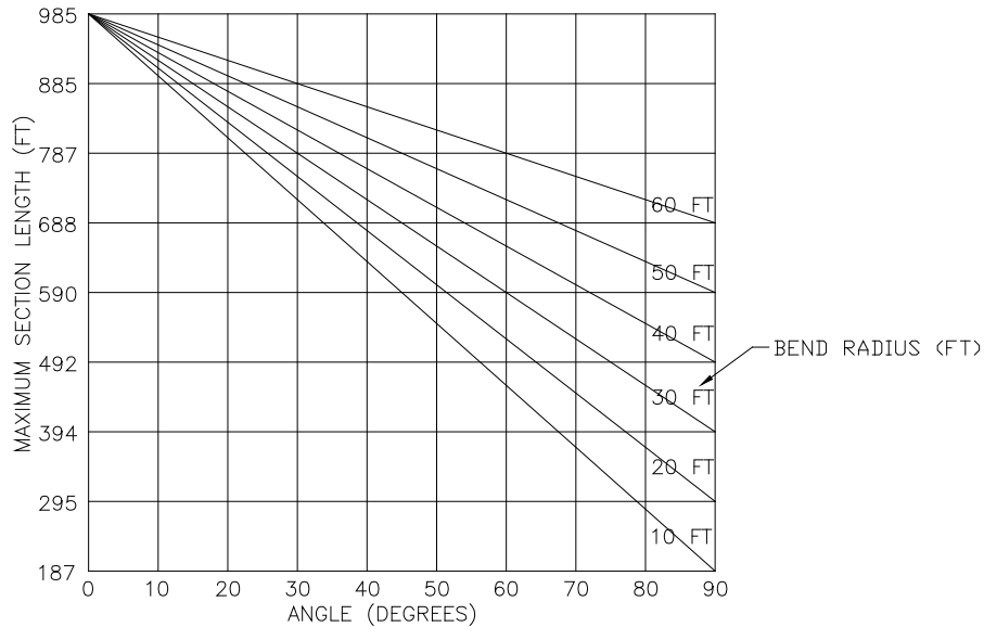
Figure G5010-1: Maximum Section Length Between Manholes
