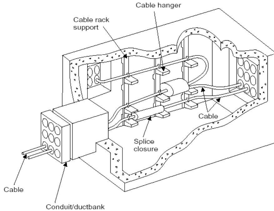
Figure G5010-2: Typical Telecommunications Manhole
