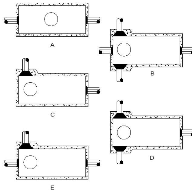
Figure G5010-3: Basic Telecommunications Manhole Configurations
