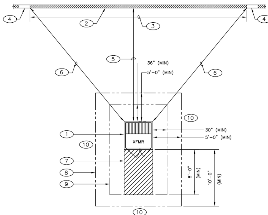
Figure G4010-1 Transformer Clearances
