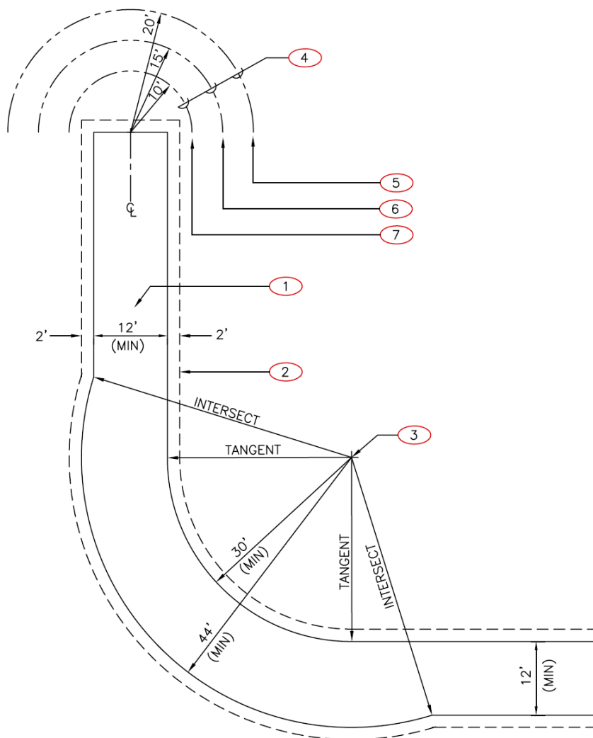
Figure G4010-2 Pad-Mounted Equipment Access Path
