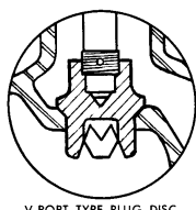
V-PORT TYPE PLUG DISC
