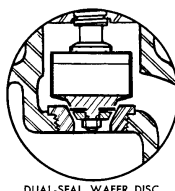
DUAL-SEAL WAFER DISC AND RENEWABLE SEAT
