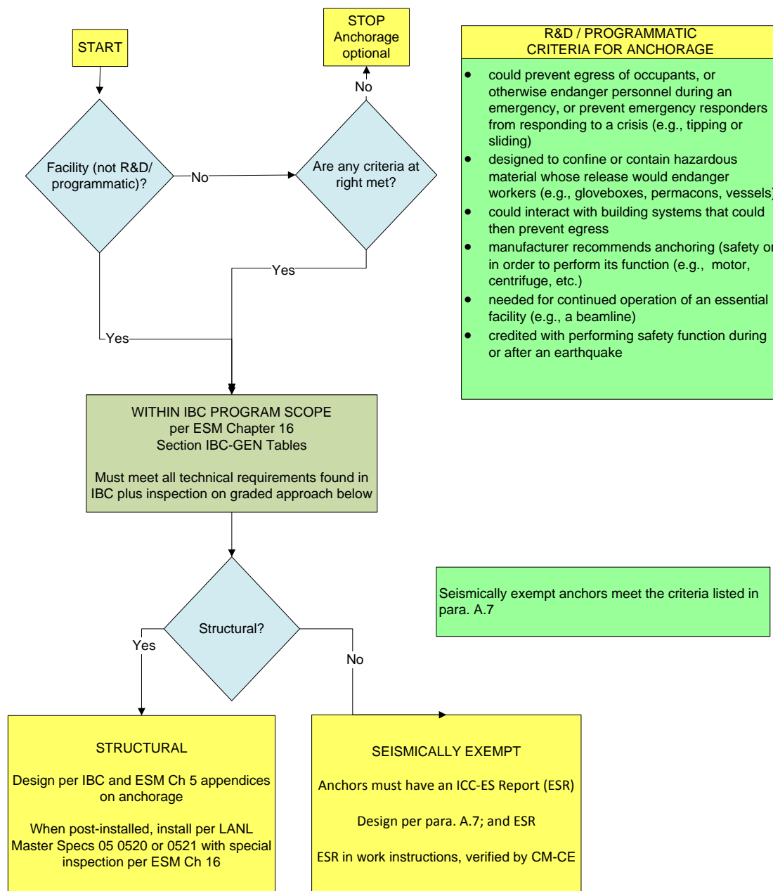
Figure II.A - 1 Non-Facility SSC Anchorage Requirements
