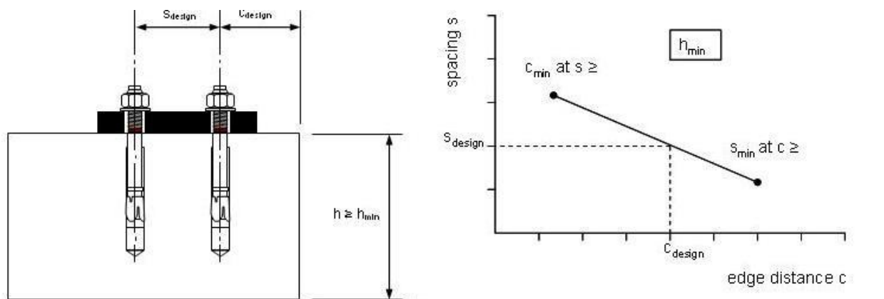
Figure III.C-3 Interpolation of Minimum Edge Distance and Minimum Spacing for KB-TZ
