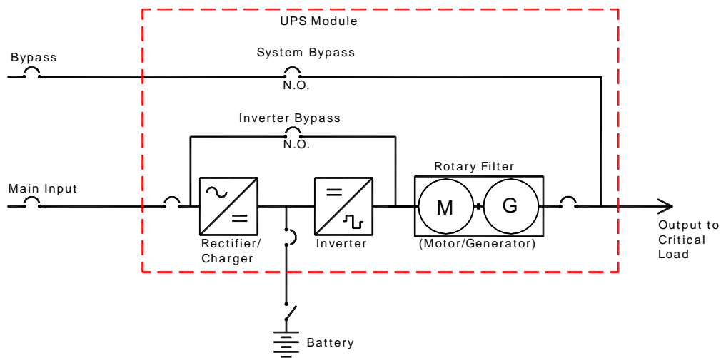
Figure D5090-2: Typical Rotary UPS System
