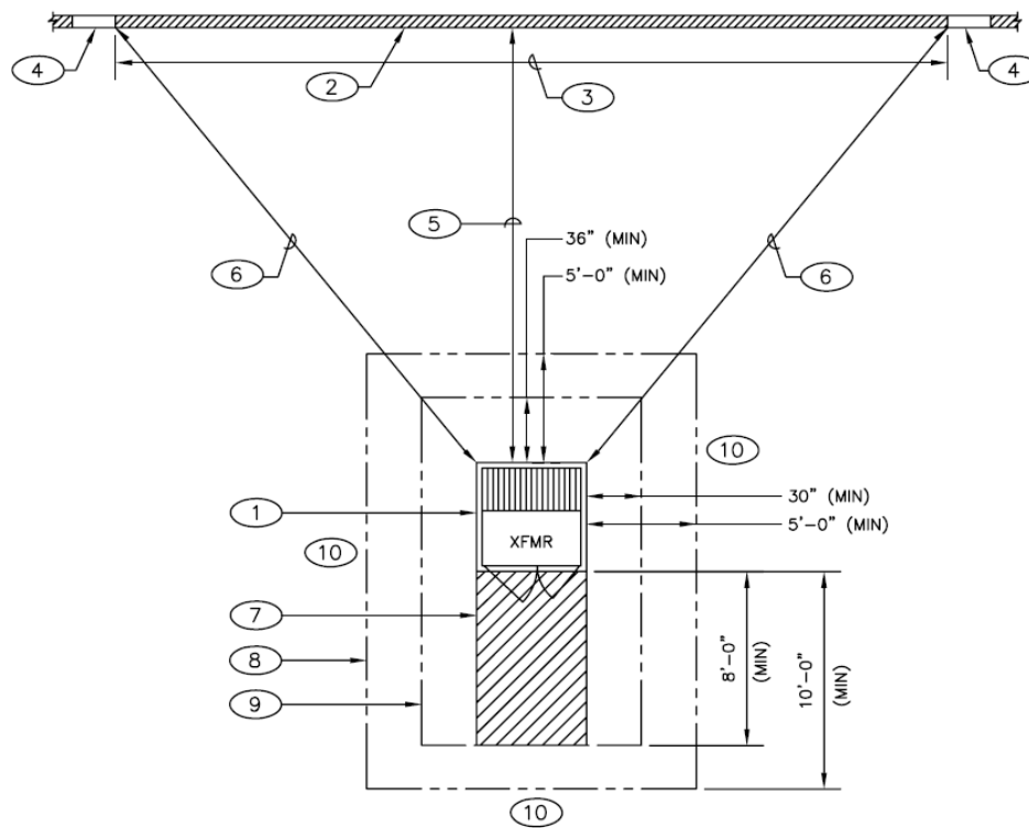
Figure G4010-1 Transformer Clearances
