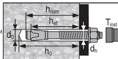
Figure 2 KB-TZ2 Installation Parameters
