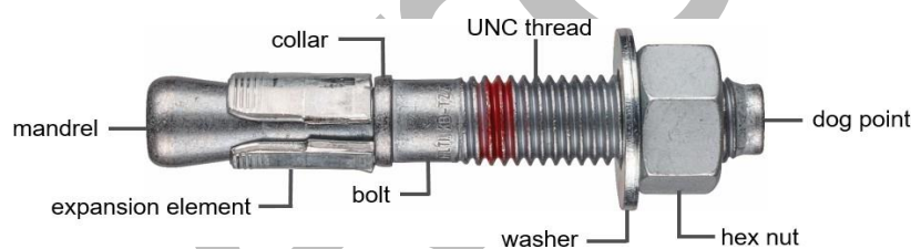
Figure 1 Kwik Bolt TZ2 (KB-TZ2)
