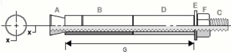
Drillco Maxi-Bolt
