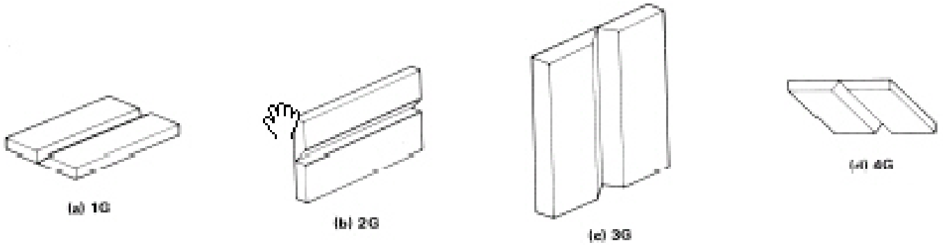
QW-461.3 GROOVE WELDS IN PLATE — TEST POSITIONS
