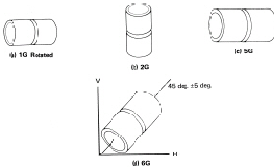
QW-461.4 GROOVE WELDS IN PIPE — TEST POSITIONS
