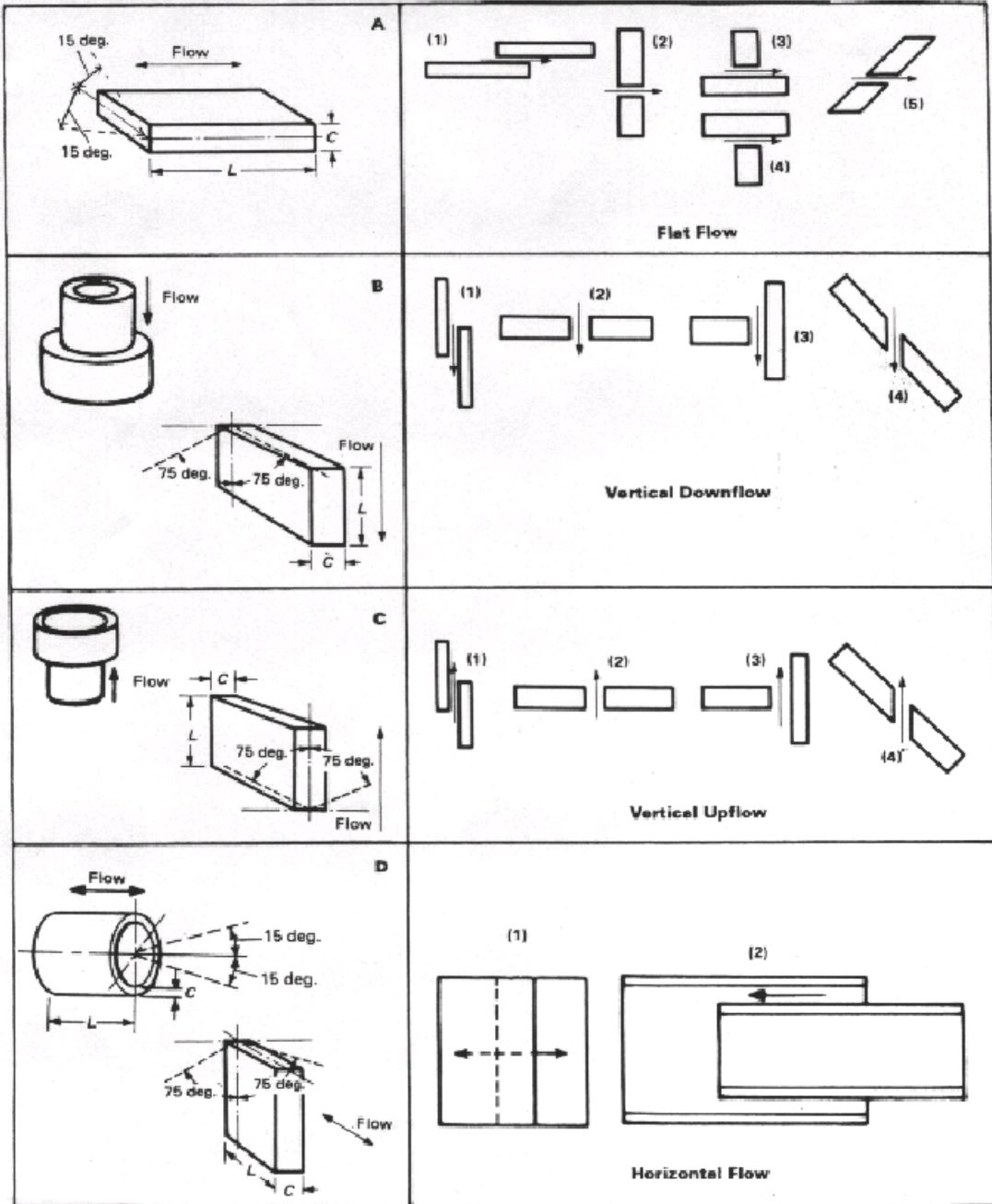
Typical brazed joints showing flow of filler metal
