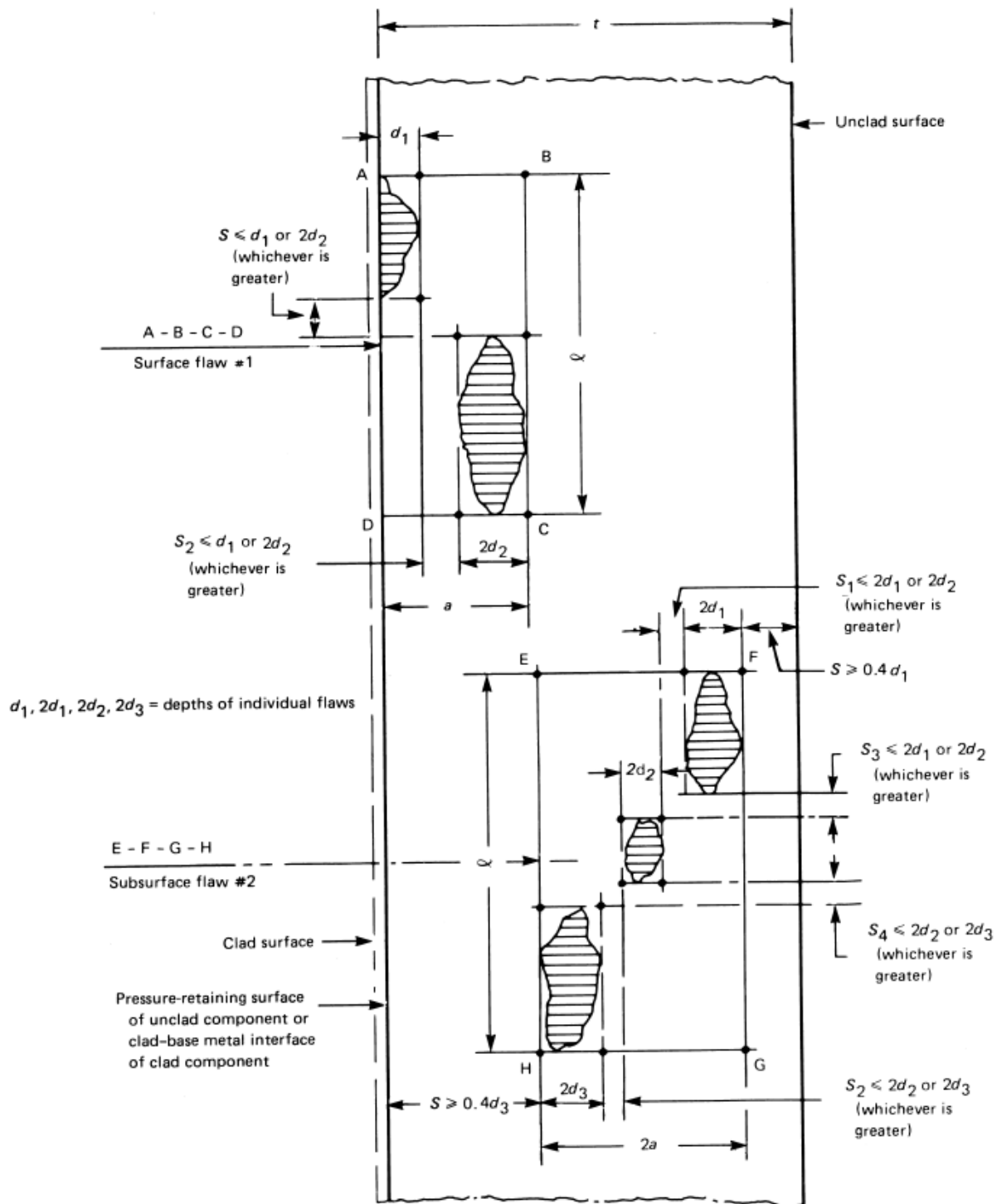
Figure KE-301-4 Nonaligned Coplanar Flaws in Plane Normal to Pressure-Retaining Surface (Illustrative Flaw Configurations)
