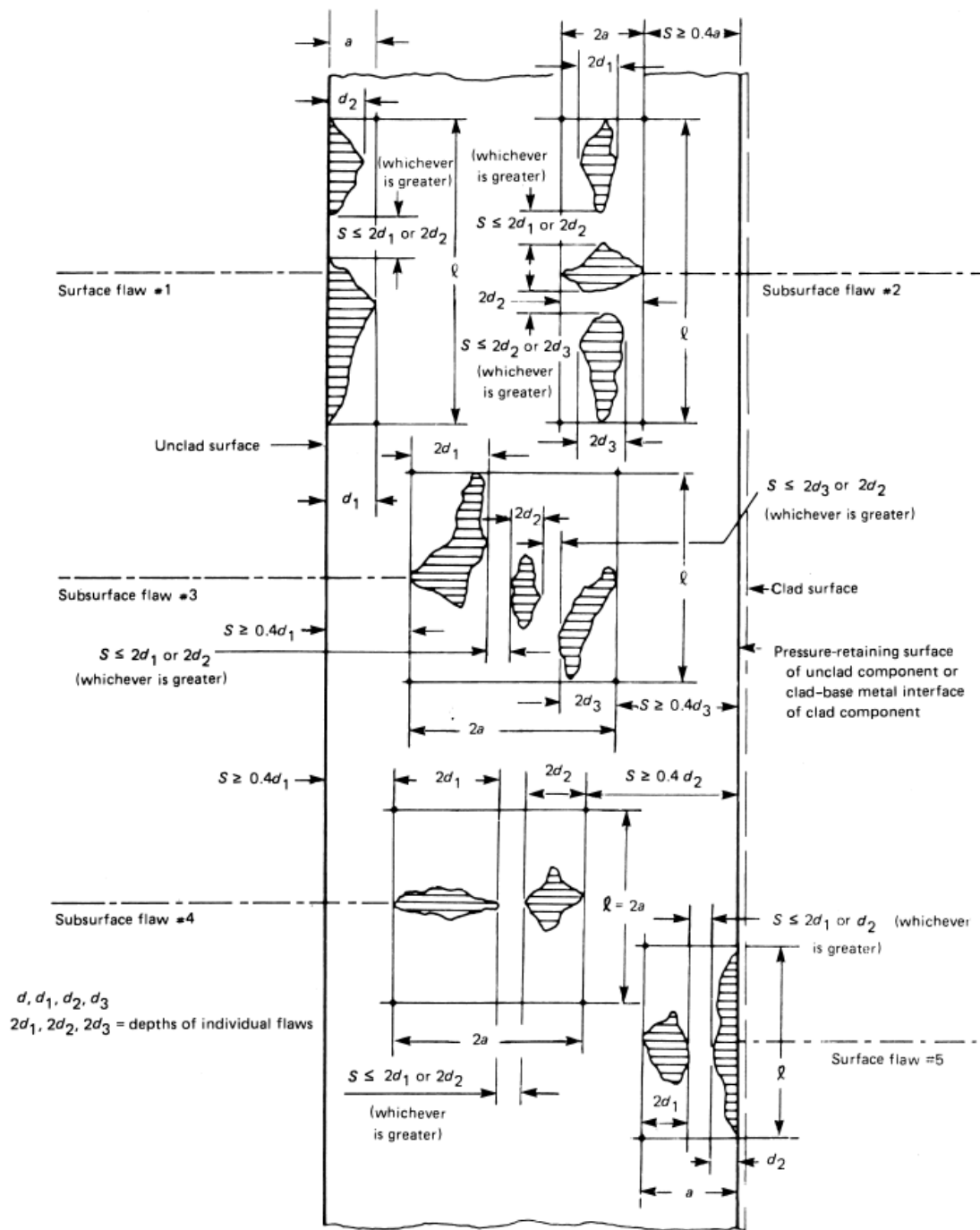
Figure KE-301-2 Multiple Planar Flaws Oriented in Plane Normal to Pressure-Retaining Surface
