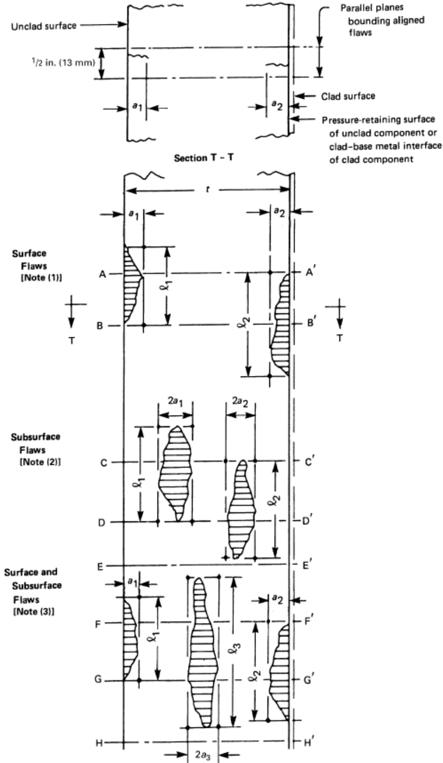
Figure KE-301-5 Multiple Aligned Planar Flaws
