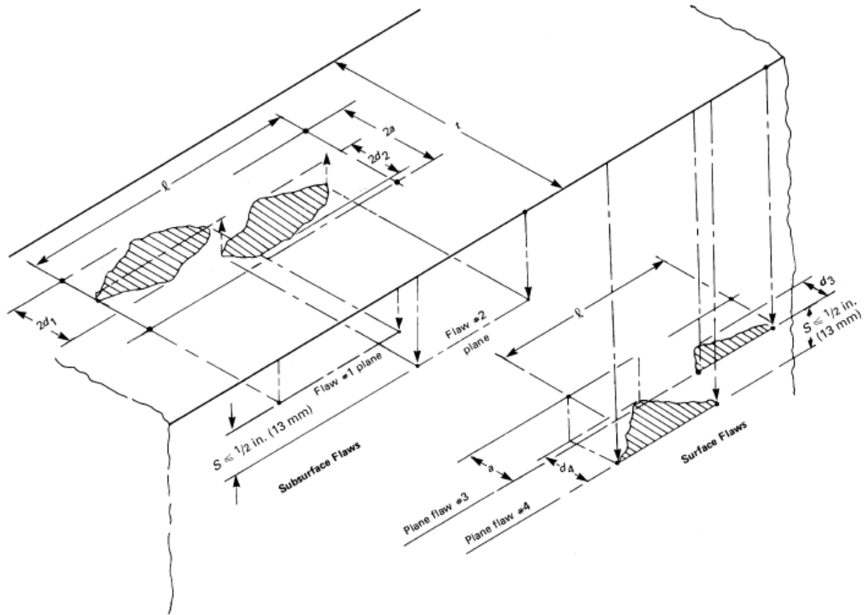
Figure KE-301-3 Parallel Planar Flaws
