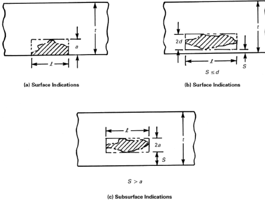
Figure KE-301-1 Single Indications
